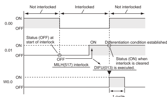
Timing chart
