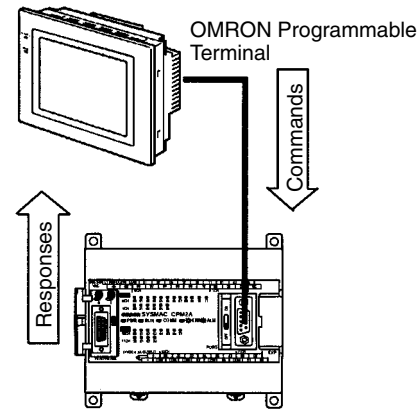
CPM2A RS-232C port connection (See note.)
